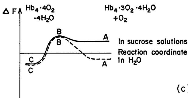
FIGURE 4 Sketches of free energy changes in reactions of hemoglobin with carbon monoxide and oxygen. Association rates are exponential functions of free energy change from A to B . Dissociation rates are exponential functions of free energy change from C to B . Equilibrium constants are exponential functions of free energy change from A to C . (a) Curves that determine k'_1 , k_1 , and K_1 . Other curves for additional CO molecules are all assumed to be similar. Hence none of these rates or equilibria are altered by CO solubility in media containing glycerol or sucrose. (b) Similar curves that determine k'_1 , k_1 , and K_1 . Curves for second and perhaps third O_2 are assumed similar in form. Hence none of these rates or equilibria are altered by changes of O_2 solubility due to sucrose or glycerol in reaction medium. (c) Curves for determination of k'_1 , k_1 , and K_1 , showing dependence of k'_1 and K_1 on solubility of O_2 .
